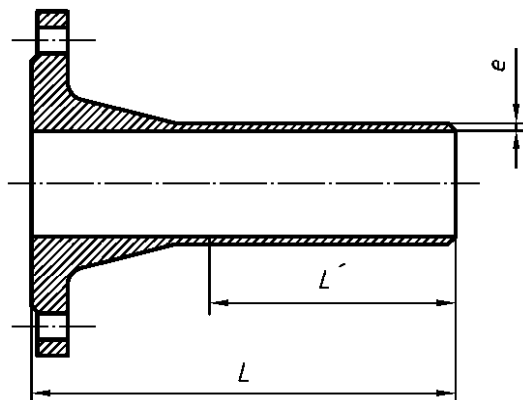
Figure 7 — Flanged spigots
