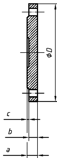
Figure 24 — Blank flanges PN 16
