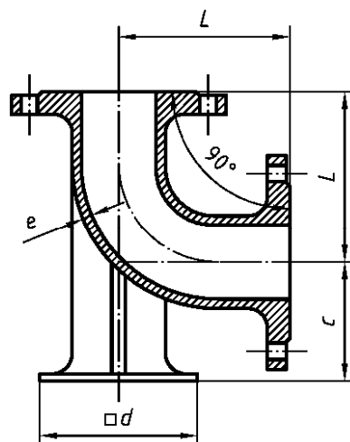
Figure 17 — Double flanged duckfoot 90° (1/4) bends
